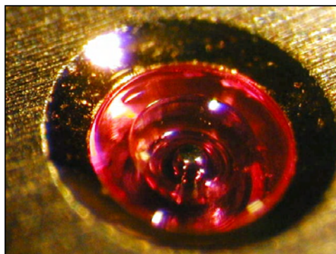
Examples showing the correct oiling of jewel holes
